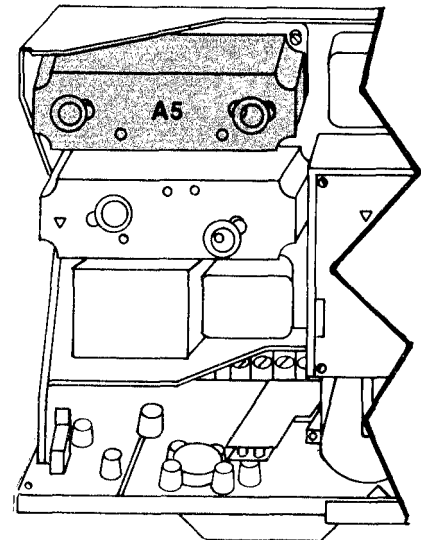
CHASSIS INTERIOR, TOP VIEW
